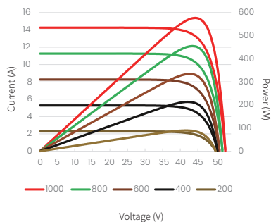
Current-Voltage & Power-Voltage Curves (585W)
